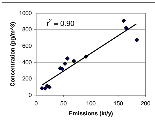
Figure 3. Correlation between global emissions of \alpha -HCH and its concentrations in arctic air with r^2 = 0.90 . The least-squares line is given by Eq. (1).
